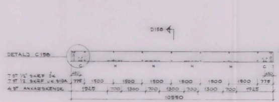
BALK 410 GB 1ST 1:50
