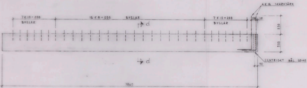
BALK B C01 H ANTAL - 1ST, B 501 H ANTAL - 1ST 1:20
