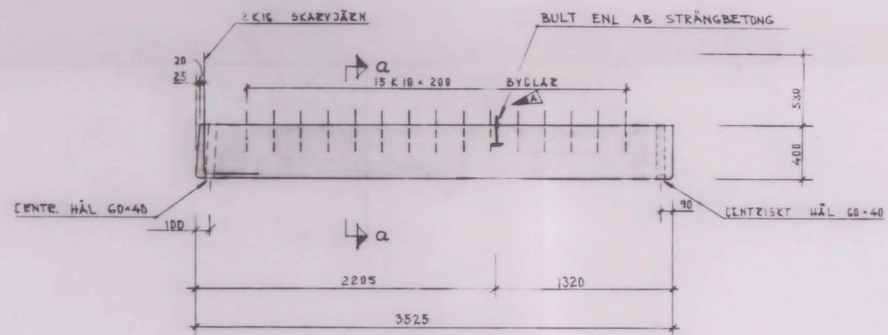
BALK B C05 H ANTAL - 1ST 1:20
