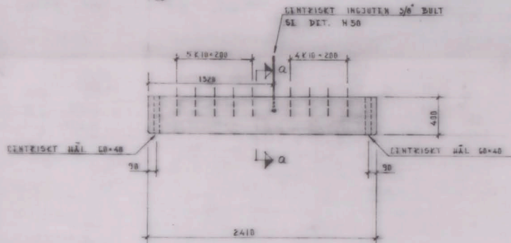
BALK B 711 H ANTAL - 1ST 1:20
